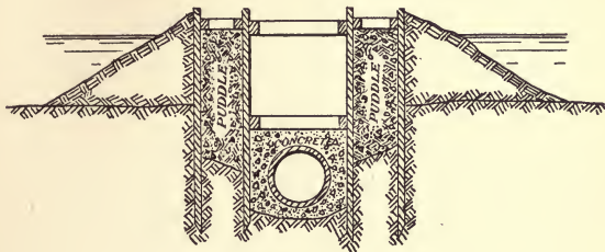
FIG. 31.—COFFER-DAM PUDDLE-WALLS.
